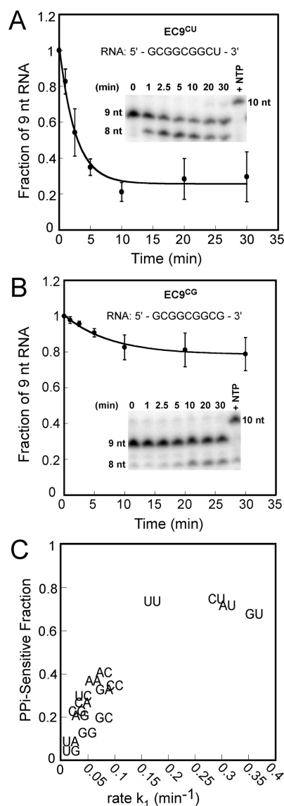
Figure 3. Identity of RNA 3' terminal nucleotide affects translocation register of Tth RNAP. (A) Quantitative analysis of pyrophosphorolysis of EC9 CU , which favors the pretranslocated state. Tth EC9 CU was reconstituted from tDNA #6059, ntDNA #5848, and RNA #6042 (Table S1). ECs (50 nM) were incubated with 0.5 mM pyrophosphate at 60 °C and disappearance of the 9 nt RNA measured at the times indicated in the inset. +NTP, UTP (1 mM) was added at the end of the time course to confirm that the unreacted EC9 CU remained active and could extend the RNA 1 nt by UMP incorporation. Errors are SD from three independent experiments. Data were fit to a simple reversible mechanism of pyrophosphorolysis (eq 3; see Materials and Methods). A value for k_1 that approximated the initial rate of pyrophosphorolysis ( 0.29 \pm 0.04 \text{ min}^{-1} ) and a final fraction of pyrophosphorolysed transcript (PPi-sensitive fraction, remaining 9-nt RNA/total RNA = 0.74 \pm 0.03 ) were determined by nonlinear regression. (B) Quantitative analysis of pyrophosphorolysis of EC9 CG , which favors the posttranslocated state. The experiment was performed identically to that shown in panel A except that Tth EC9 CG was reconstituted from tDNA #6062, ntDNA #5848, and RNA #6045 (Table S1). (C) A plot of fraction of EC susceptible to pyrophosphorolysis (PPi-sensitive fraction) with 0.5 mM PPi versus the rate of pyrophosphorolysis for 16 combinations of 3'-proximal dinucleotide sequence.
