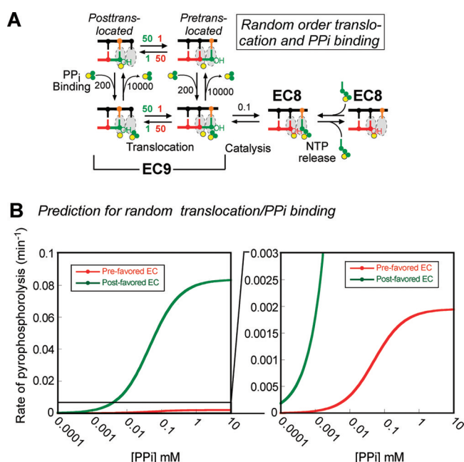
Figure 9. Random order of translocation of PPi binding/release can explain differences in pyrophosphorolysis of EC9 UG and EC9 GU . (A) A random-order translocation and PPi binding/release mechanism. With the arbitrarily chosen rate constants shown in the figure, the mechanism can account for a V_{\max} difference with little effect on apparent K_{\text{PPi}} . Translocation rates were assigned based on translocation bias of a particular EC. Forward and backward translocation rate constants for prefavored ECs are shown in green (50 and 1 s -1 , respectively), whereas those for postfavored ECs are in red (1 s -1 ; forward rate constant; 50 s -1 : reverse rate constant). (B) A kinetic simulation graph of pretranslocation-favoring EC9 GU (green) and posttranslocation favoring EC9 UG (red) ECs was generated using the reaction scheme shown in (A) using the program KinTek Global Kinetic Explorer (see Materials and Methods).
