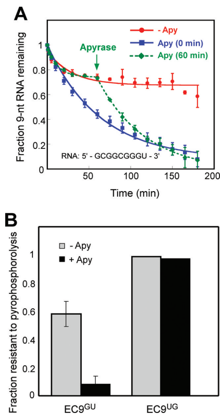
Figure 4. Incomplete pyrophosphorolysis by Eco RNAP is caused by NTP accumulation. (A) Rates of pyrophosphorolysis of Eco EC9 GU . Eco EC9 GU reconstituted using E. coli RNAP and the pretranslocation favoring scaffold (#6063, #5848, #6046; Table S1). Eco EC9 GU (50 nM) was incubated at 37 °C with 0.5 mM PPi alone (red), in the presence of 0.5 U apyrase/mL (blue), or with addition of apyrase to 0.5 U/mL 60 min after the reaction was initiated (green) for the time indicated. Samples were removed at the times indicated and the fraction EC9 GU remaining was plotted as a function of time. The error bars represent standard deviations obtained from four different experiments. The data from reaction without apyrase (red) are fit to a simple reversible mechanism of pyrophosphorolysis (eq 3; see Materials and Methods), whereas data from reaction with apyrase (blue) are fit to a single exponential for a pseudo-first-order reaction. (B) Fraction of Eco EC9 GU and Eco EC9 UG resistant to pyrophosphorolysis at 0.5 mM PPi in the absence (gray) or presence (black) of apyrase.
