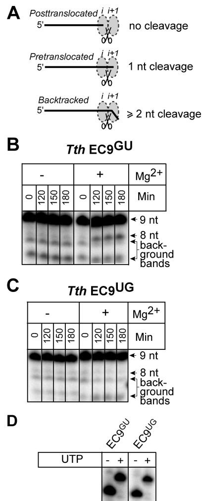
Figure 6. Pyrophosphorolysis-resistant Tth EC9 UG is not backtracked. (A) Predicted outcomes for intrinsic cleavage reactions of pretranslocated, posttranslocated, and backtracked ECs. Posttranslocated ECs does not generate cleavage products, whereas pretranslocated and backtracked complexes produce 1-nt cleavage products and 2 or more cleavage products, respectively. (B) Intrinsic cleavage reaction of Tth EC9 GU . Tth EC9 GU was reconstituted using Tth RNAP and the pretranslocation-favoring scaffold (#6063, #5848, #6046; Table S1) containing 5' end 32 P-labeled RNA at pH 9 without Mg 2+ . Intrinsic cleavage reaction was initiated by the addition of 20 mM Mg 2+ , and samples were removed and separated by electrophoresis at the times indicated (see Materials and Methods). (C) Intrinsic cleavage reaction of Tth EC9 UG . Tth EC9 UG was reconstituted and assayed as in panel A except with the posttranslocation-favoring scaffold (#6070, #5848, #6053; Table S1). (D) EC9 GU and EC9 UG were incubated with 100 \mu M UTP to extend their respective RNAs by one nucleotide, thus showing the ECs were active and not arrested.
