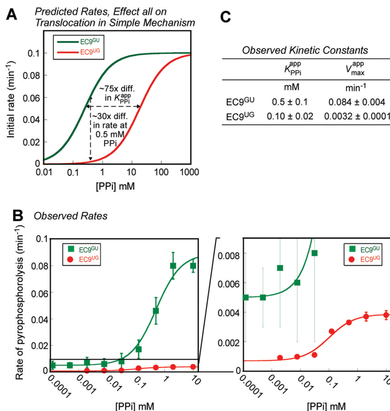
Figure 8. PPi concentration dependence of pyrophosphorolysis in Eco EC9 GU and Eco EC9 UG . (A) A predicted relationship for the rate of pyrophosphorolysis vs [PPi] for the ordered translocation/PPi binding mechanism shown in Figure 6A and Figure 1. The difference in apparent K_{PP_i} (~75×) between EC9 GU and EC9 UG and in rate at 0.5 mM PPi concentration are indicated on the plot. (B) Kinetic analysis of [PPi] dependence of pyrophosphorolysis in EC9 GU and EC9 UG . Rate of pyrophosphorolysis for Eco EC9 GU and Eco EC9 UG over a wide range of PPi concentrations. (C) Approximate, apparent kinetic constants of EC9 GU and EC9 UG are calculated from the plot shown in (B) (see Materials and Methods).
