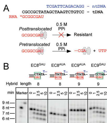
Figure 2. Pyrophosphorolysis by Tth RNAP on a minimal scaffold. (A) A representative example of a minimal nucleic acid scaffold used in this study (yields EC8^{AU} ). *, 5'\text{-}^{32}\text{P} . The color scheme for RNA and DNA is the same as in Figure 1A. The posttranslocated state is resistant to pyrophosphorolysis; the pretranslocated state is competent for pyrophosphorolysis, yielding UTP in this case. (B) ECs containing Tth RNAP were assembled on four minimal nucleic acid scaffolds that differ only in the sequence shown above the gel panels. The time course of pyrophosphorolysis (0.5 mM PP_i ) at 60 °C is shown, with the sizes of RNAs indicated.
