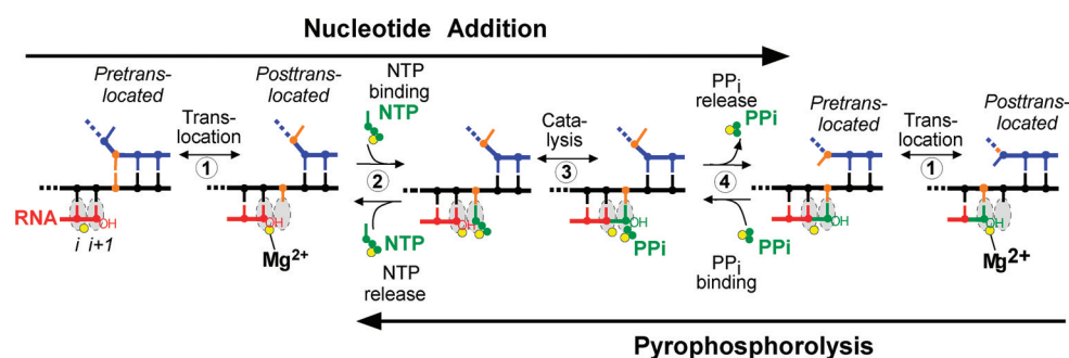
Figure 1. Nucleotide addition and pyrophosphorolysis cycle. Template DNA is shown in black, nontemplate DNA in blue, RNA in red, incoming nucleotide triphosphate and pyrophosphate in green, and Mg^{2+} in yellow. One template/nontemplate position is colored orange to illustrate translocation. The EC alternates between pre- and posttranslocated states with the RNA 3' nt in the i or i + 1 subsites, prior to NTP binding (step 1). NTPs enter the active site when the EC is posttranslocated (step 2). Catalysis (step 3) requires a rate-limiting conformational change in which the trigger loop folds into the trigger helices (not shown). Release of PP_i (step 4) completes the nucleotide addition cycle. Pyrophosphorolysis is the reverse reaction of nucleotide addition. Since catalysis itself is reversible, net pyrophosphorolysis requires that the thermodynamic driving force of PP_i conversion to NTP + RNA^{1-} exceed the conversion of NTP to PP_i + RNA^{1+} . Pyrophosphorolysis requires the EC be in the pretranslocated register, but whether PP_i binding/release and translocation occur with obligate order is not established.
