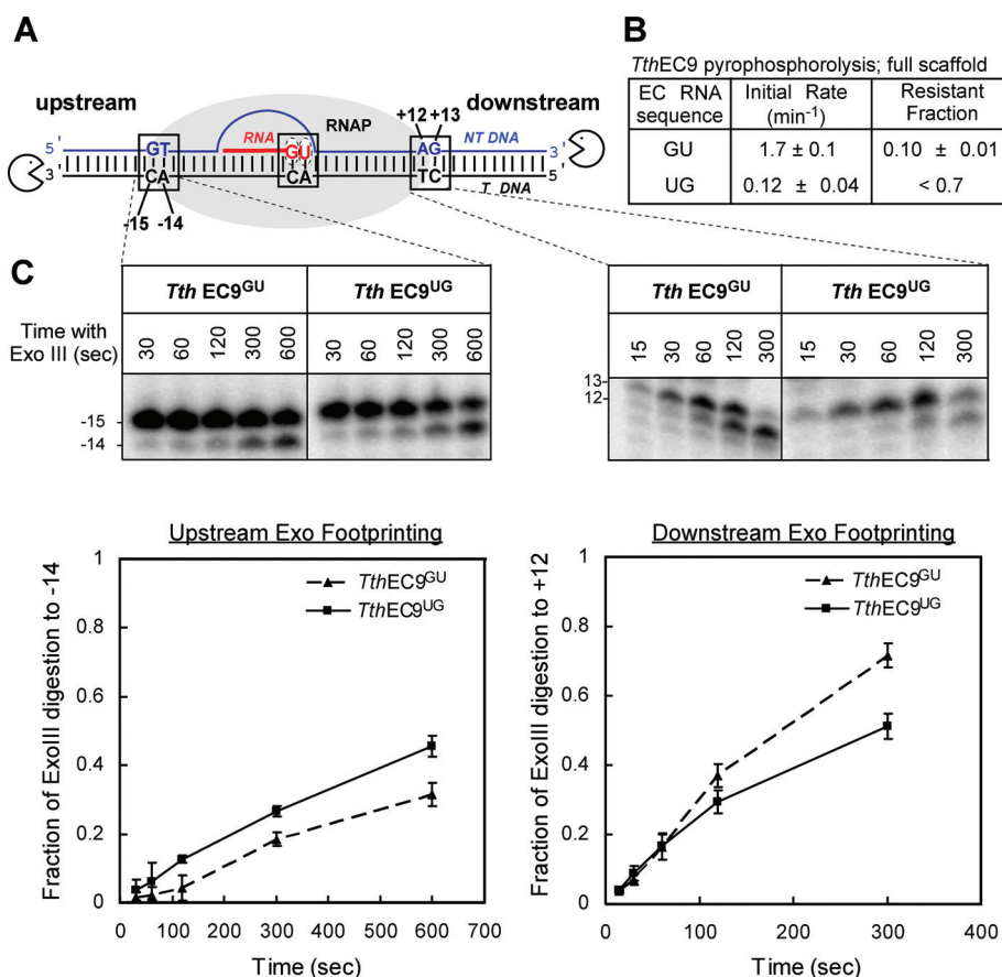
Figure 5. ExoIII footprints of TthEC9 GU (pretranslocated) and TthEC9 UG (posttranslocated). (A) Schematic of the complete scaffold used for exoIII footprinting experiments. The sizes of the template DNA (upstream) and the nontemplate DNA (downstream) fragments protected by RNAP from digestion by ExoIII are illustrated. For the nontemplate strand assay, the nontemplate strand contained a 5' 32 P label and the template strand contained a 3' phosphorothioate bond. For template strand assay, the template strand contained a 5' 32 P label and the nontemplate strand contained a 3' phosphorothioate bond. (B) Pyrophosphorolysis results of EC9 GU and EC9 UG on complete scaffolds used for ExoIII footprinting experiments. The RNA and template DNA (GU: #6046, #6355; UG: #6053, #6357; Table S1) were first annealed, then mixed with Tth RNAP, and then annealed to the nontemplate strand (GU: #6354; UG: #6356; Table S1; see Materials and Methods). ECs (50 nM) were incubated with 0.5 mM PPi at 60 °C. The initial rate of pyrophosphorolysis ( k_1 ) and the fraction resistant to pyrophosphorolysis were determined as described in Materials and Methods. (C) Upstream ExoIII footprinting (left) and downstream ExoIII footprinting (right) of EC9 GU and EC9 UG . Plot on the left depicts the appearance of the nontemplate DNA -14 band, which should be faster when the pretranslocated register is favored. Plot on the right depicts the appearance of the template DNA +12 band, which should be faster when the posttranslocated register is favored.
