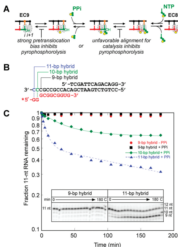
Figure 7. RNA 3' dinucleotide UG is not intrinsically resistant to pyrophosphorolysis by Eco RNAP. (A) Translocation bias toward posttranslocated state or a slow catalysis could account for the insensitivity of EC9 UG . (B) Nucleic acid scaffolds with different potential RNA:DNA hybrid length. RNA is shown in red; template and nontemplate DNA strands are in black. The 9-bp, 10-bp, and 11-bp potential RNA:DNA hybrid are created by varying the length of template DNA without changing the length of the 11-nt RNA (the template DNAs in 9-bp, 10-bp, and 11-bp hybrids end at the positions marked with a black line, a green, or a blue line, respectively). RNA was labeled with 32 P at its 5' end (*). (C) Plot of pyrophosphorolysis of ECs reconstituted with Eco RNAP and different scaffolds shown in Figure 6B. ECs were incubated with 0.5 mM PPI, 0.5 U apyrase/mL at 37 °C for the times indicated. Representative gel panels for EC9 UG (9-bp hybrid) and EC11 UG (11-bp hybrid) are shown in the inset. "C", chase lane in which ECs were chased with 1 mM UTP at the end of pyrophosphorolysis time course (after 3 h).
